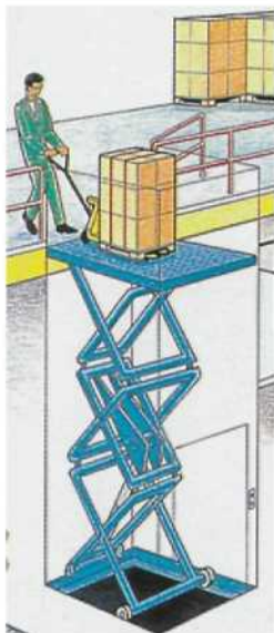
2 ton hydraulic goods platform Size 3300 x 2700 mm for use at Yamaha Motors warehouse
